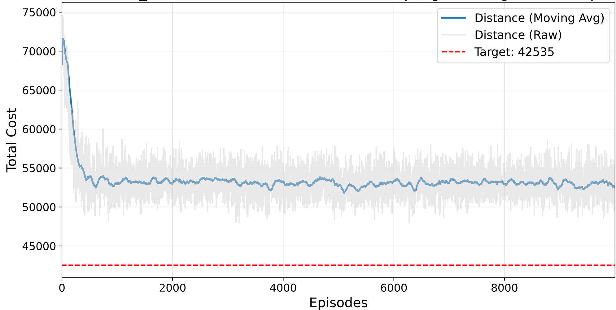
Final NO_MASK Masked AutoRL-SOP (Resampling) Training - ft70.3.sop
